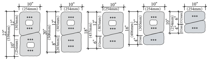
UNIT ABOVE VERTICAL UNIT SPANS TO BEAR ON EACH SIDE. VERTICAL UNITS - 6" x 12" (152mm x 305mm)
